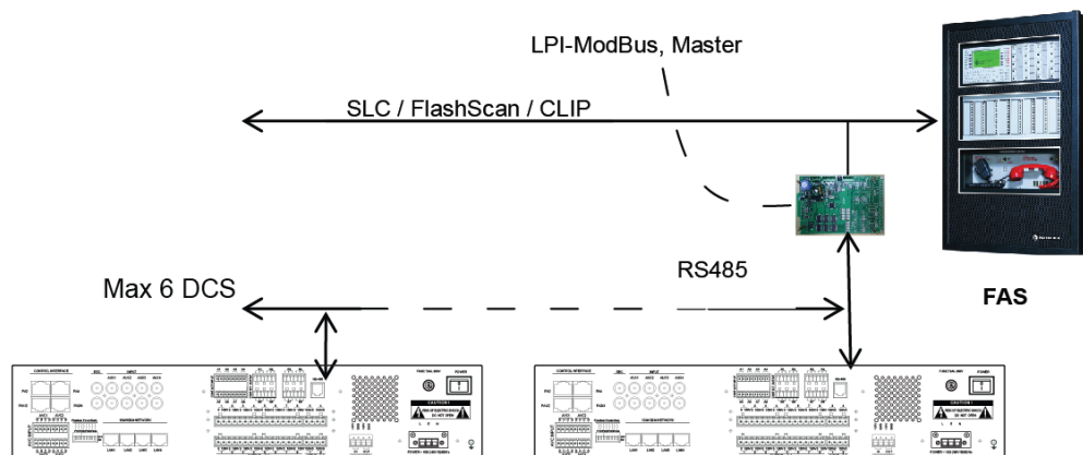
Figure 26 Schematic Diagram of Connecting DCS with Fire Alarm Control Panel through LPI-ModBus
